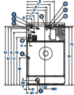
BACK ELEVATION
